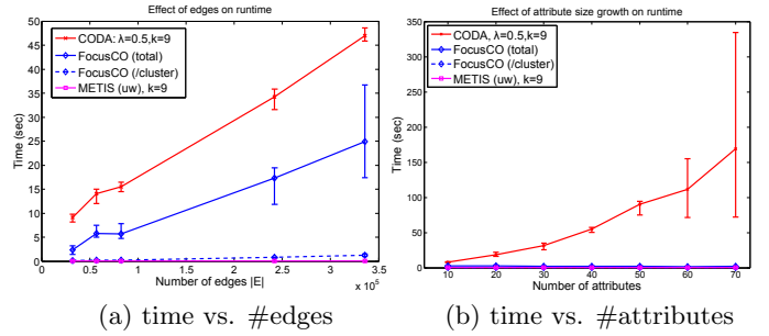
Figure 7: Running time scalability w.r.t. (a) number of edges |E| and (b) number of attributes |F| .
